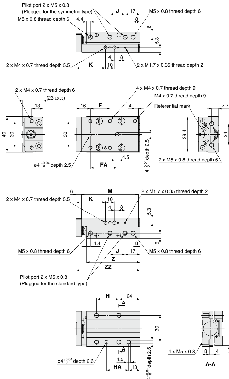
Locating pin hole geometry for positioning the body (Same dimensions on the other side)
